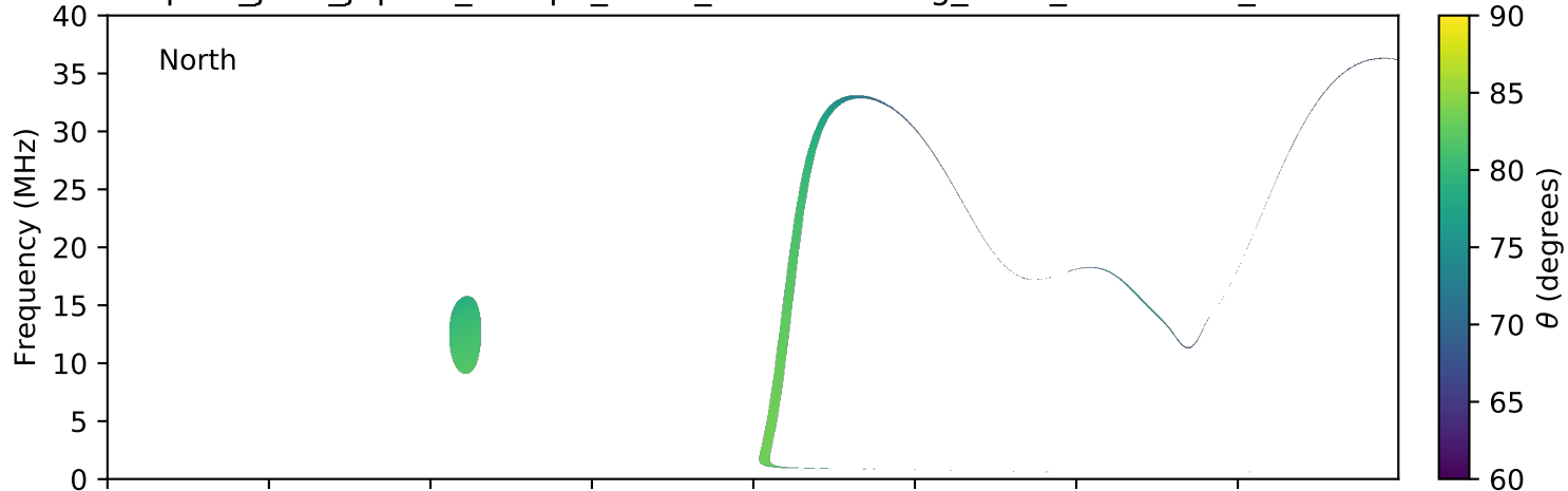
expres_juno_jupiter_europa_isaac_lossc-wid1deg_3kev_20160102_v01.cdf
