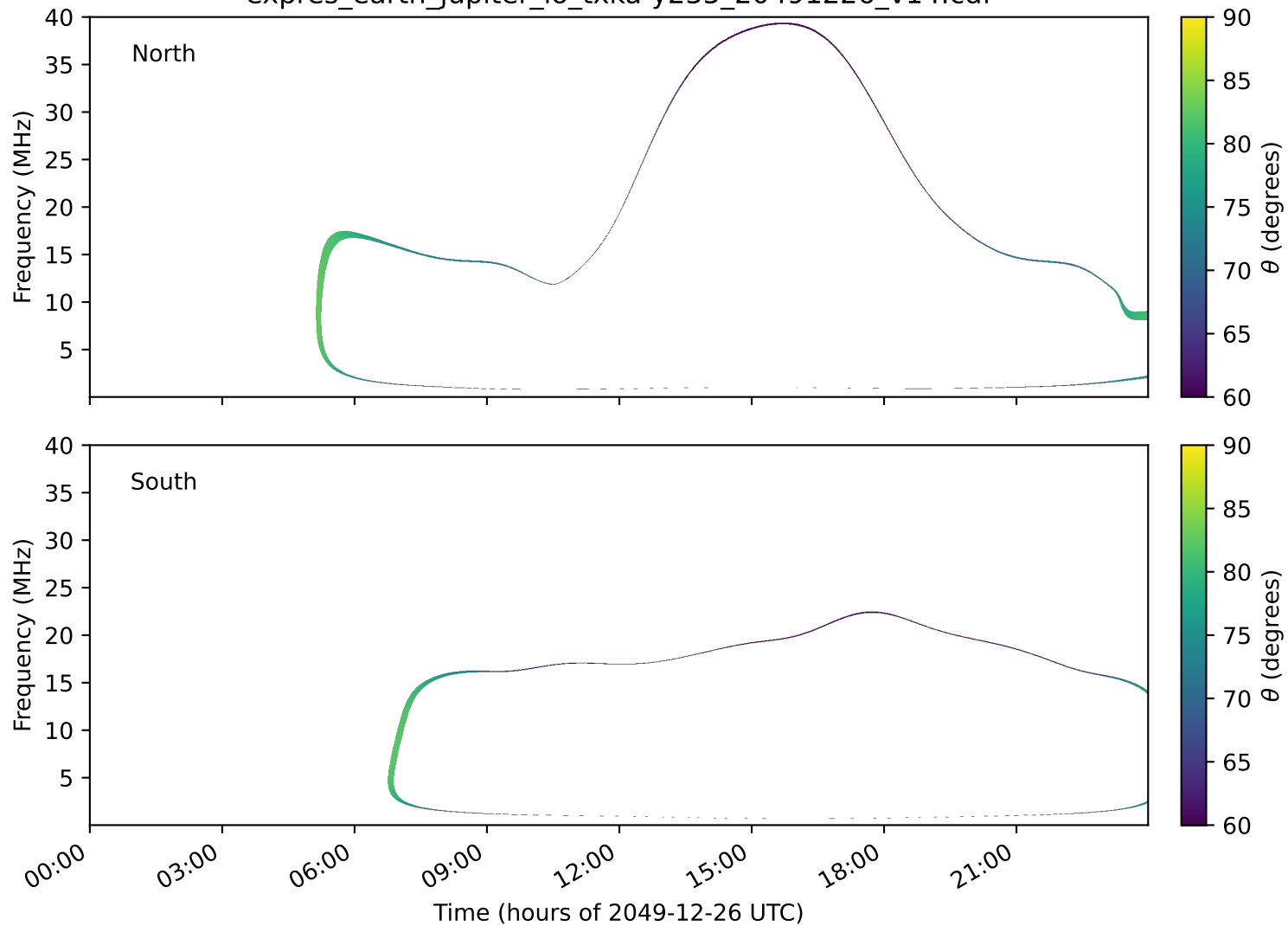
expres_earth_jupiter_io_txka-y235_20491226_v14.cdf
