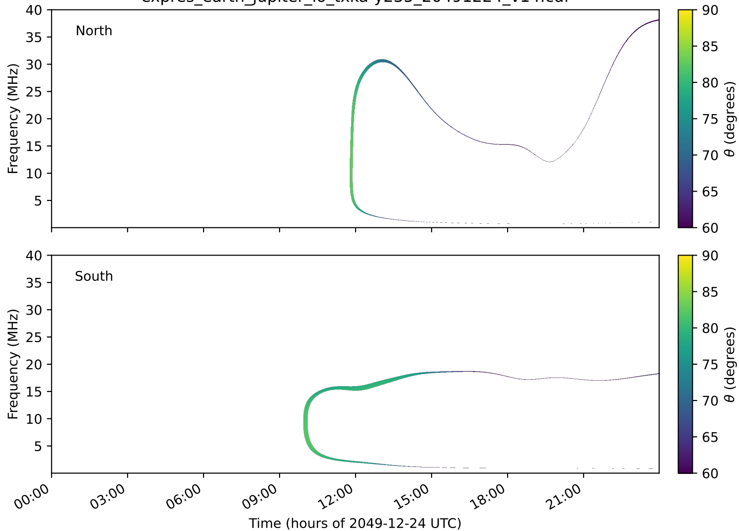
expres_earth_jupiter_io_txka-y235_20491224_v14.cdf
