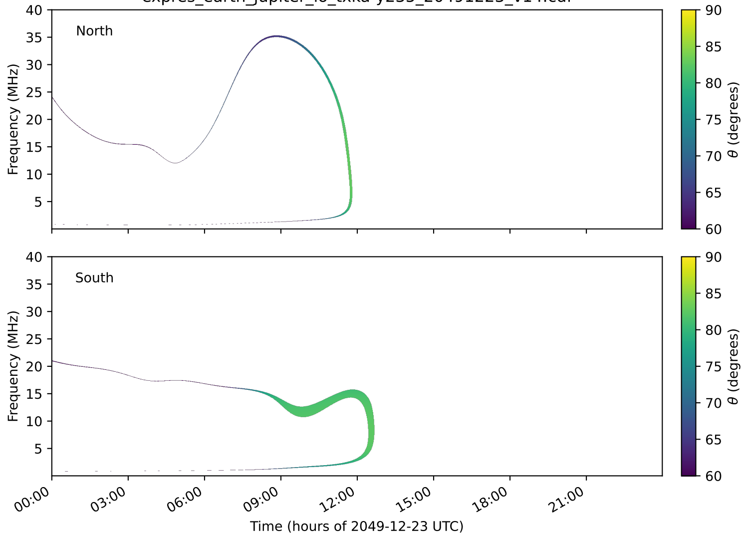
expres_earth_jupiter_io_txka-y235_20491223_v14.cdf
