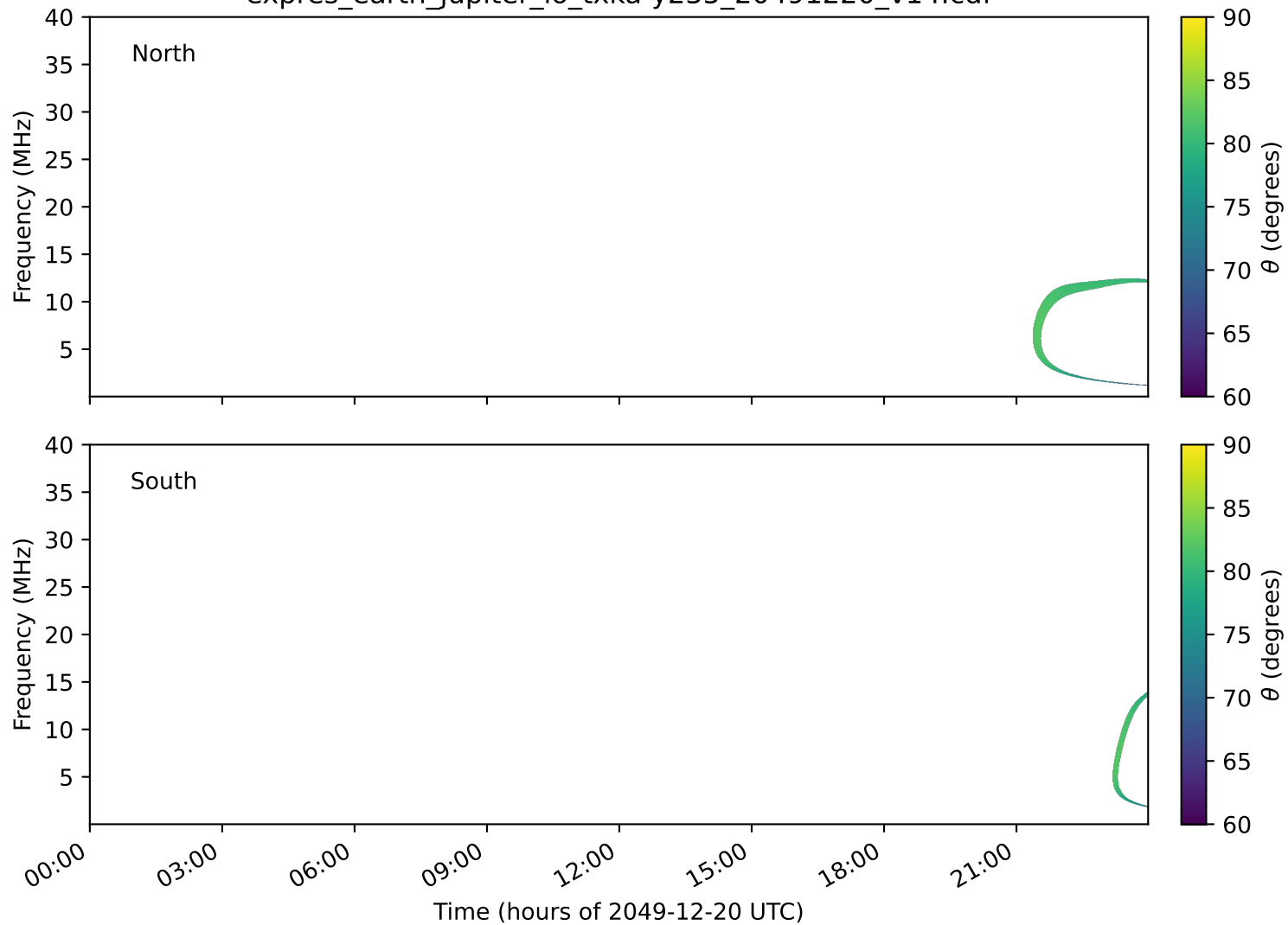
expres_earth_jupiter_io_txka-y235_20491220_v14.cdf
