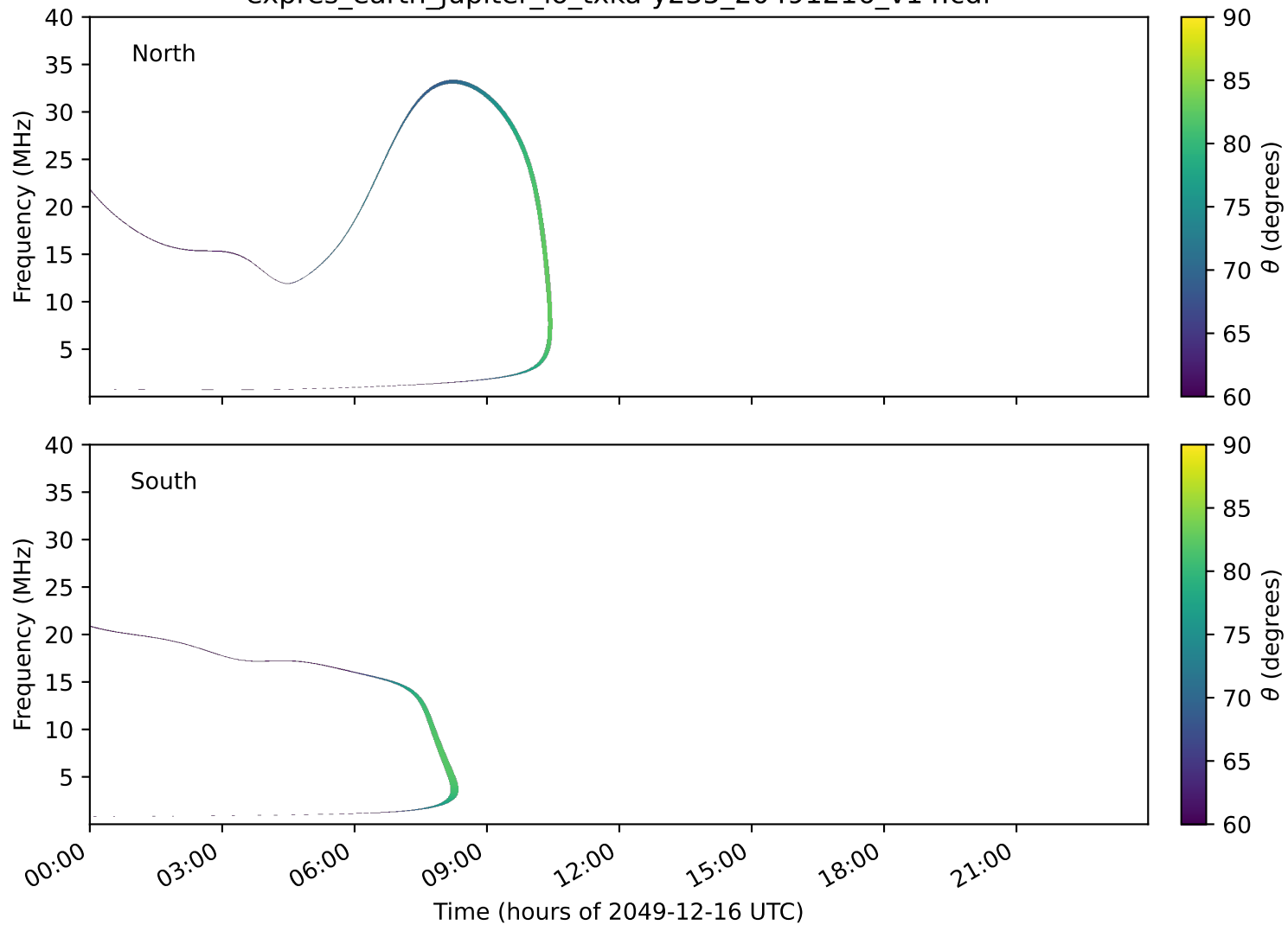
expres_earth_jupiter_io_txka-y235_20491216_v14.cdf
