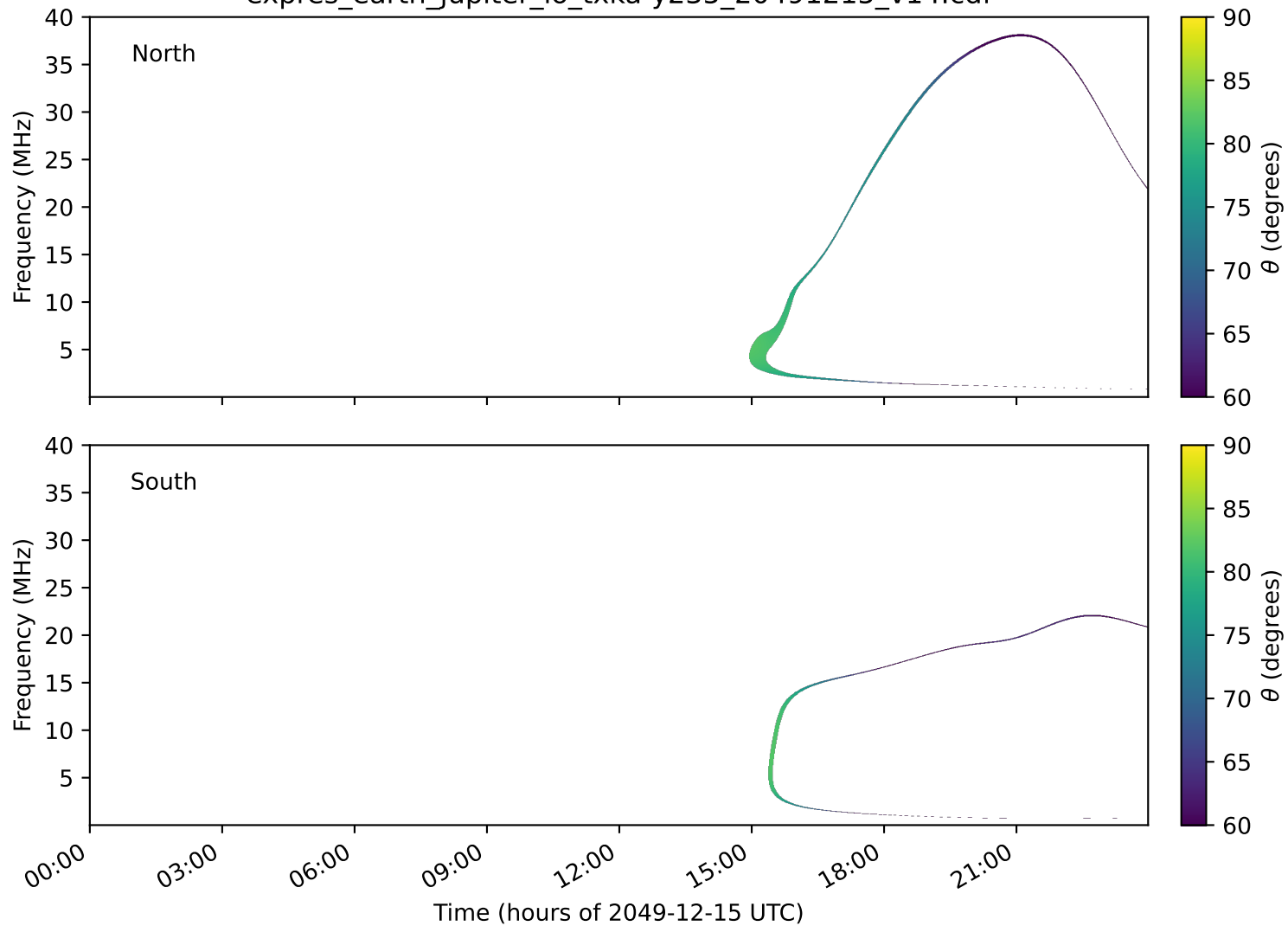
expres_earth_jupiter_io_txka-y235_20491215_v14.cdf
