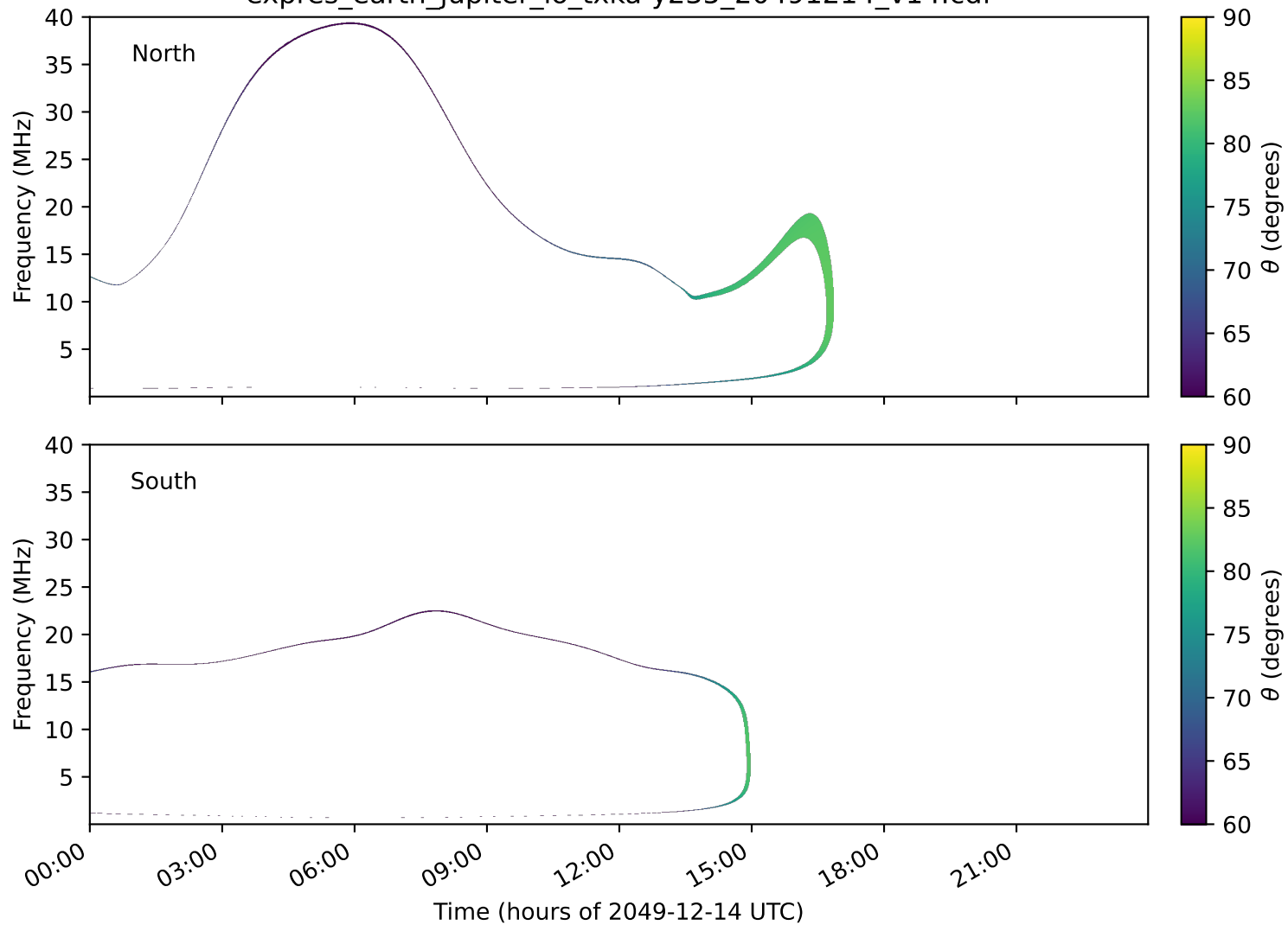
expres_earth_jupiter_io_txka-y235_20491214_v14.cdf
