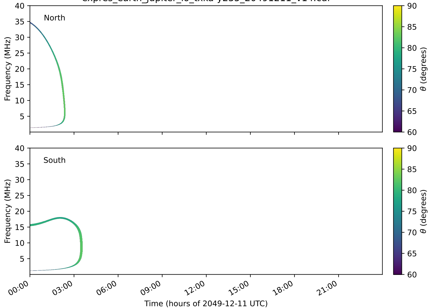
expres_earth_jupiter_io_txka-y235_20491211_v14.cdf
