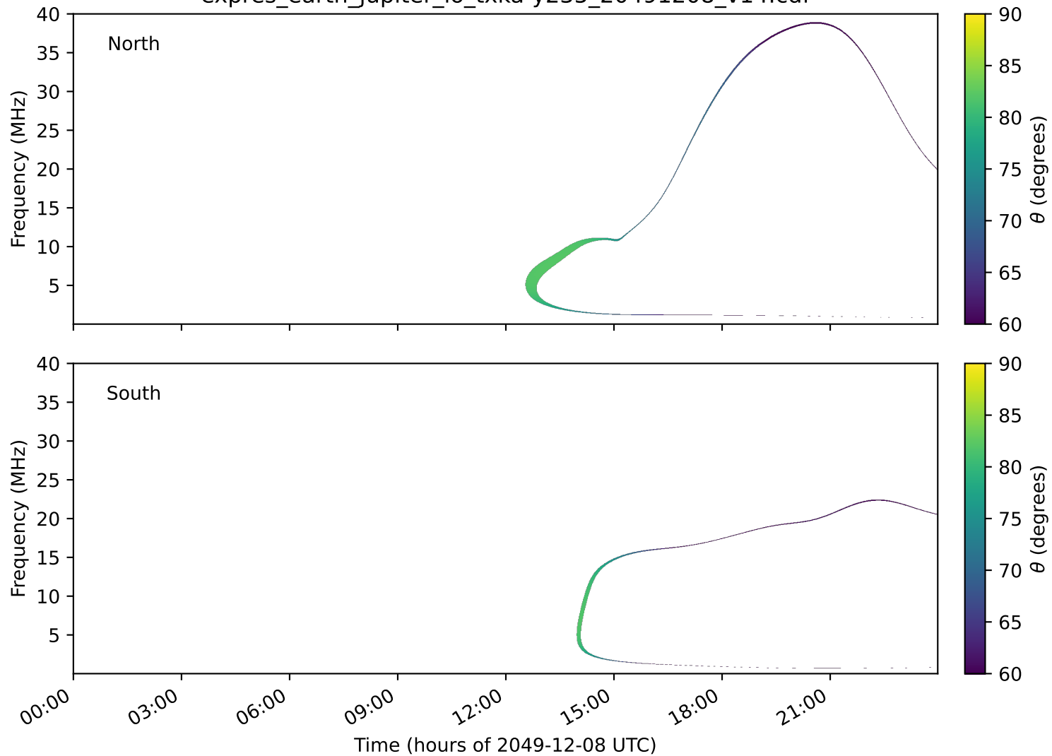
expres_earth_jupiter_io_txka-y235_20491208_v14.cdf
