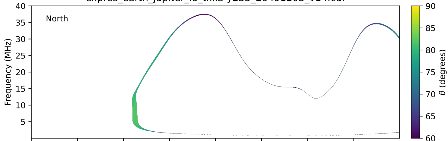
expres_earth_jupiter_io_txka-y235_20491203_v14.cdf
