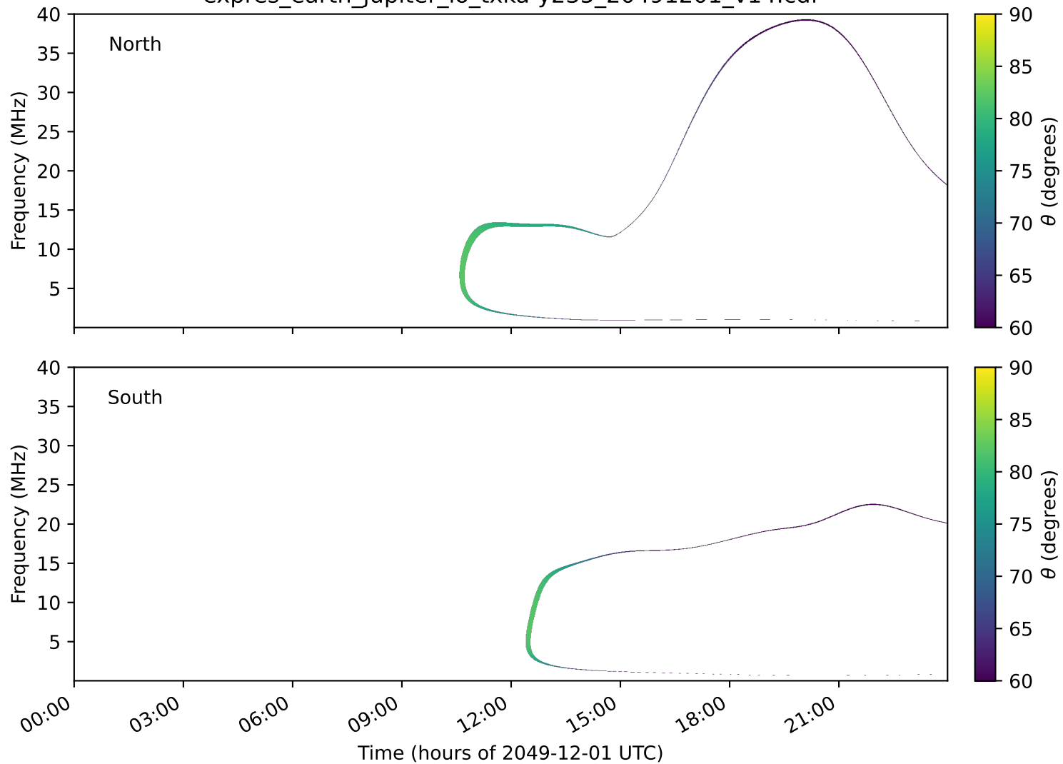
expres_earth_jupiter_io_txka-y235_20491201_v14.cdf
