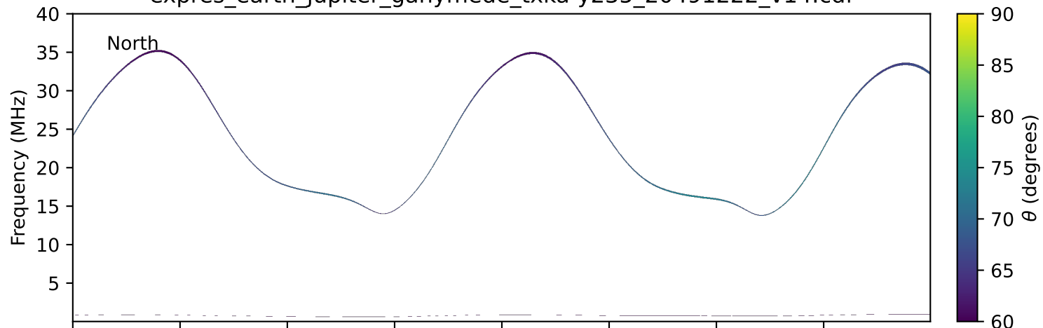
expres_earth_jupiter_ganymede_txka-y235_20491222_v14.cdf
