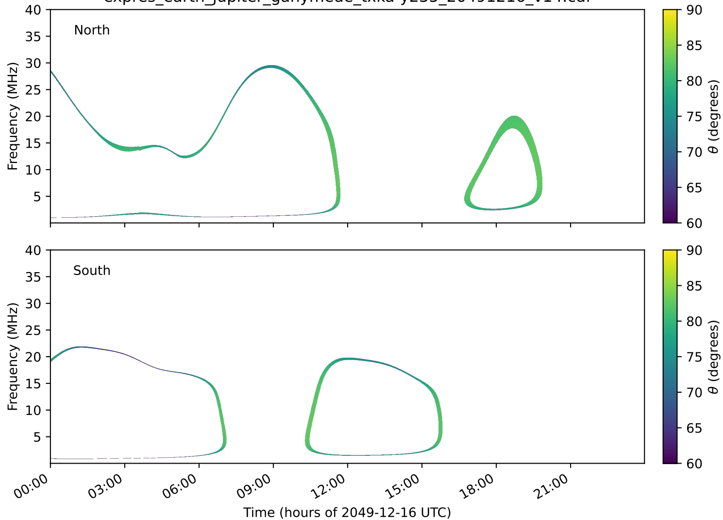
expres_earth_jupiter_ganymede_txka-y235_20491216_v14.cdf
