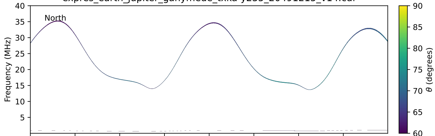
expres_earth_jupiter_ganymede_txka-y235_20491215_v14.cdf
