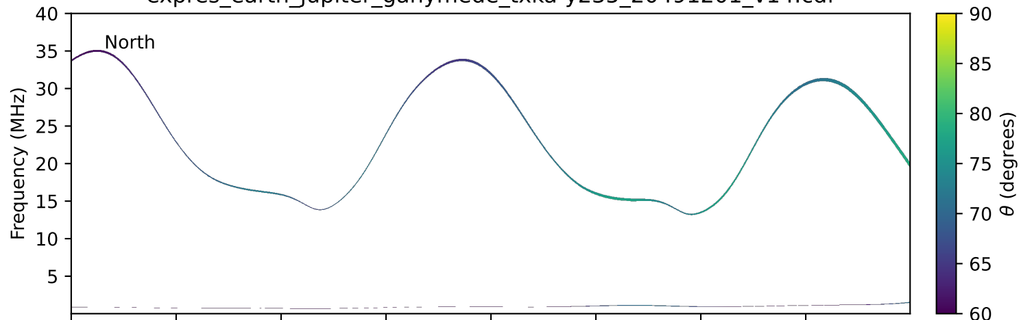
expres_earth_jupiter_ganymede_txka-y235_20491201_v14.cdf
