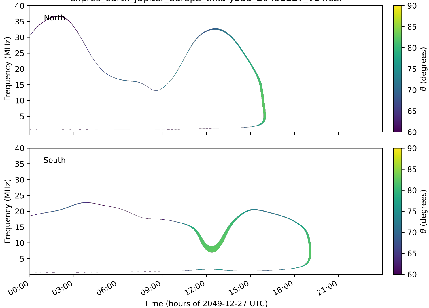
expres_earth_jupiter_europa_txka-y235_20491227_v14.cdf
