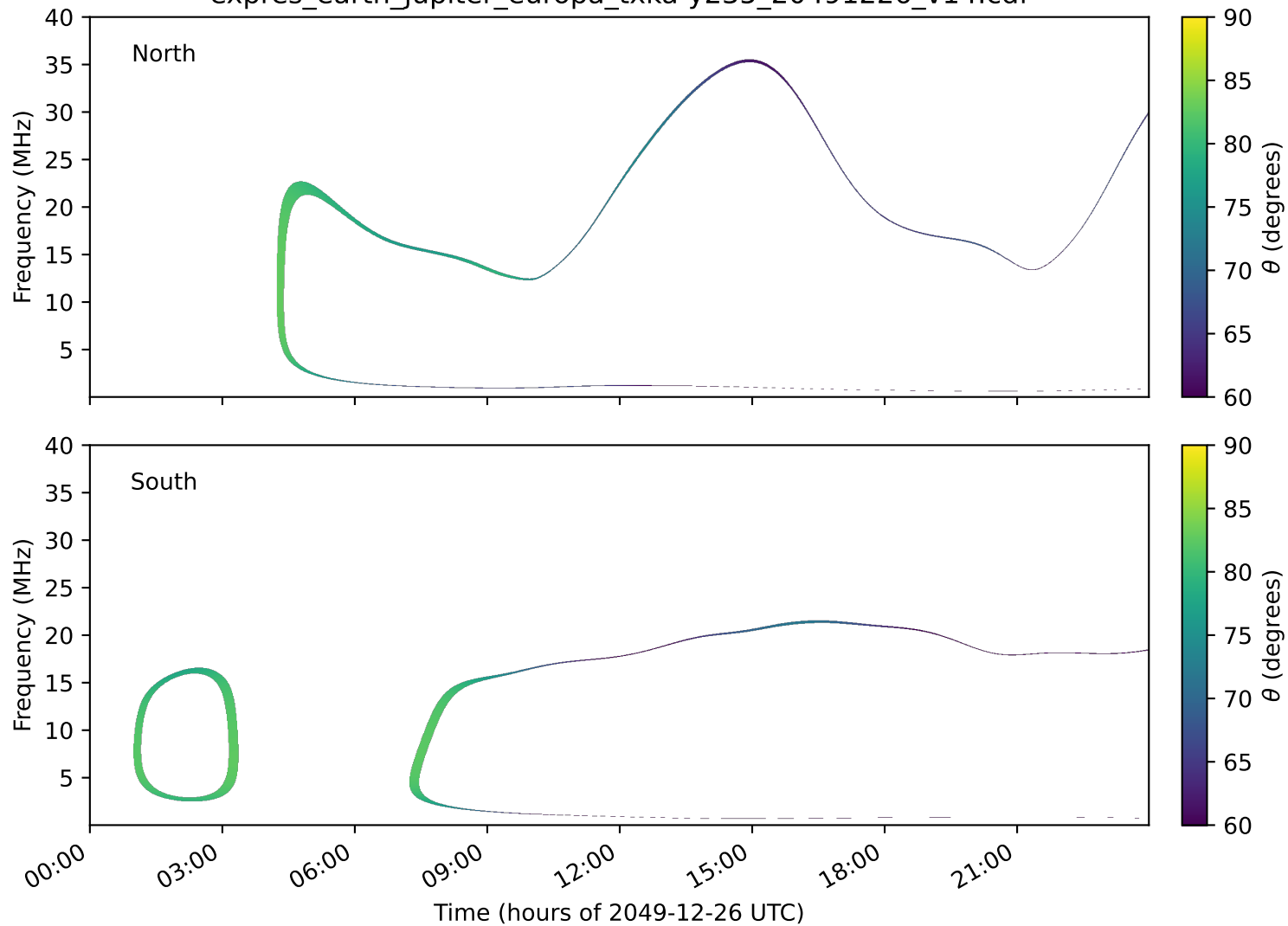
expres_earth_jupiter_europa_txka-y235_20491226_v14.cdf
