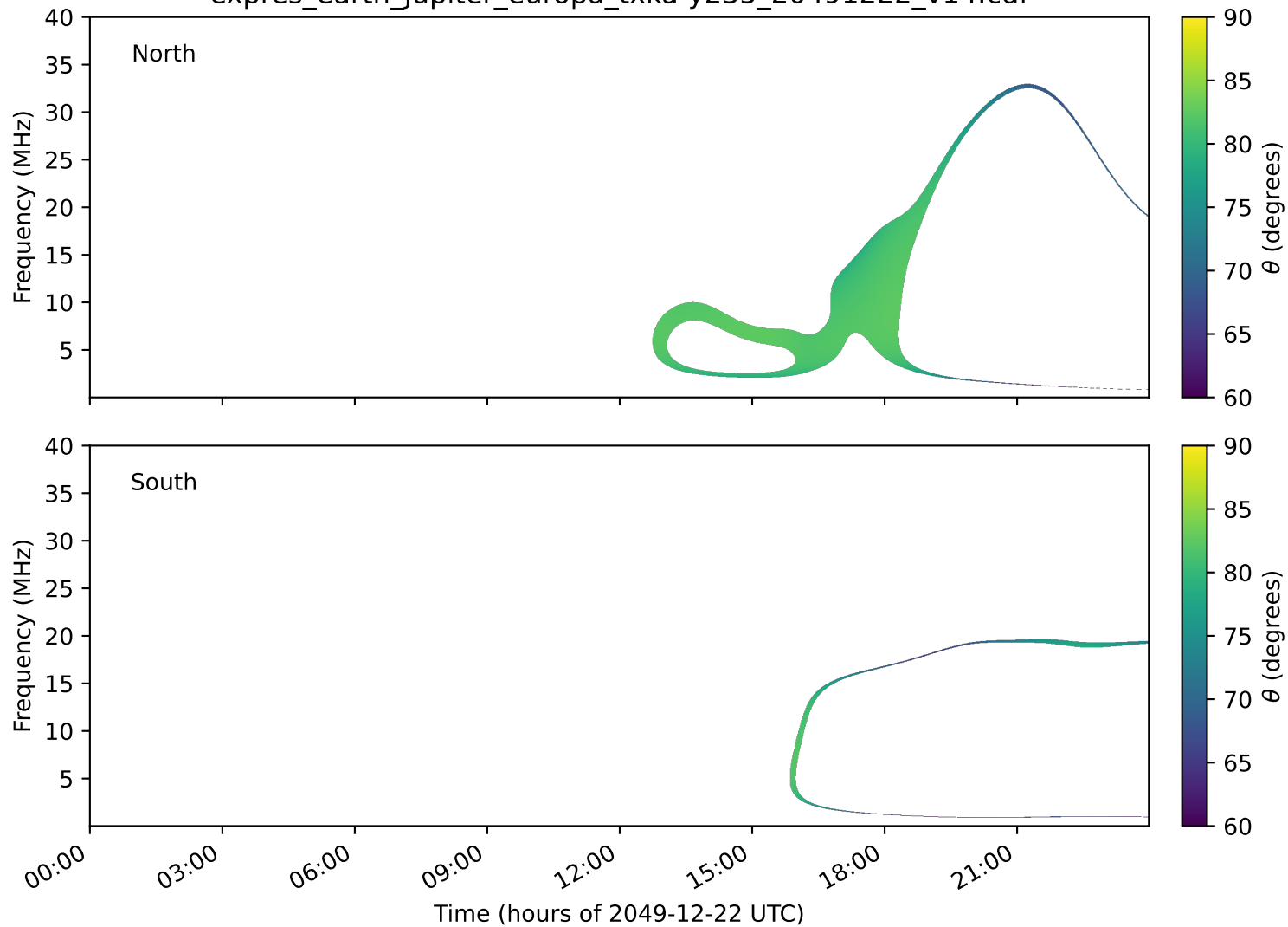
expres_earth_jupiter_europa_txka-y235_20491222_v14.cdf
