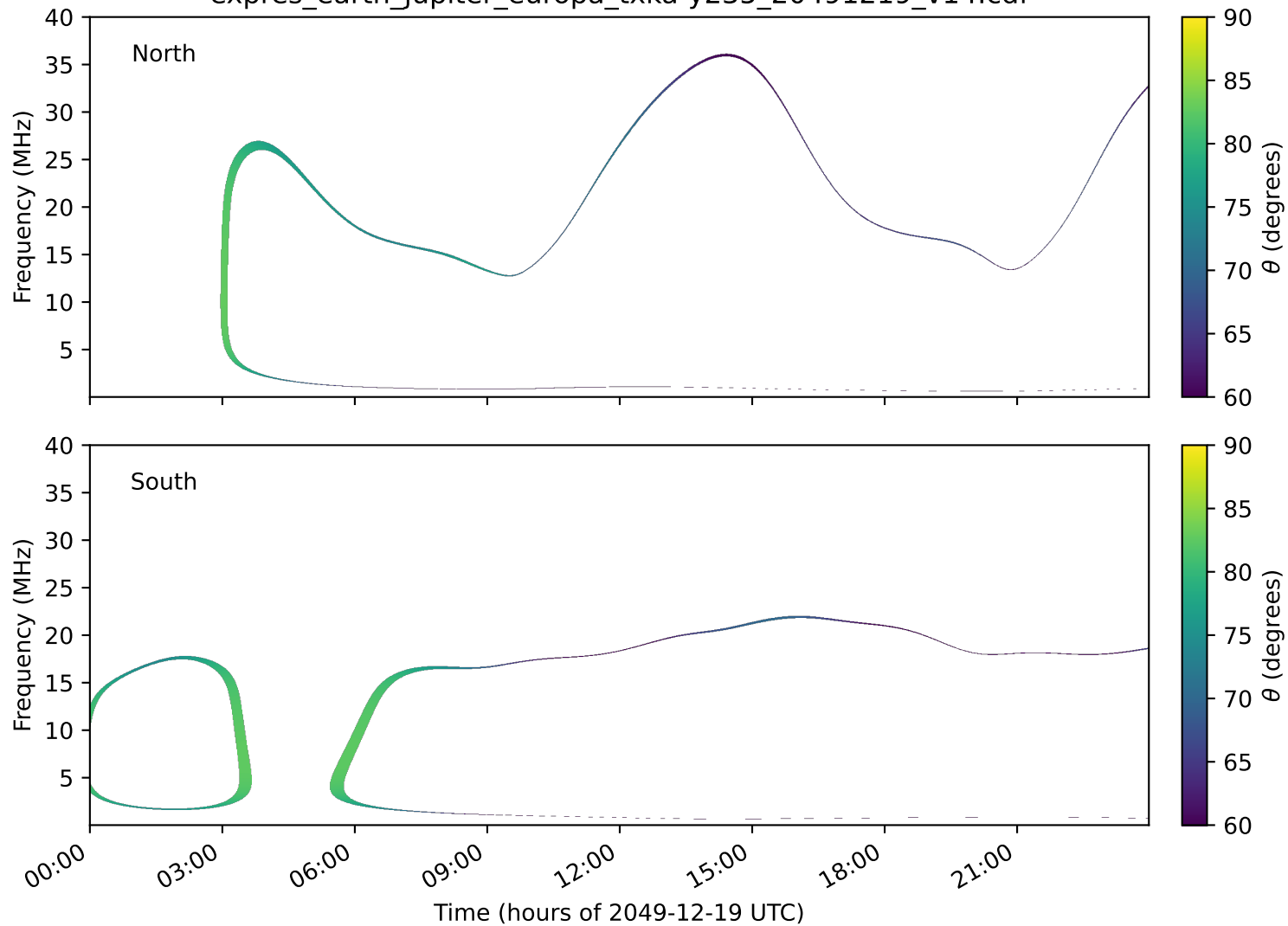
expres_earth_jupiter_europa_txka-y235_20491219_v14.cdf
