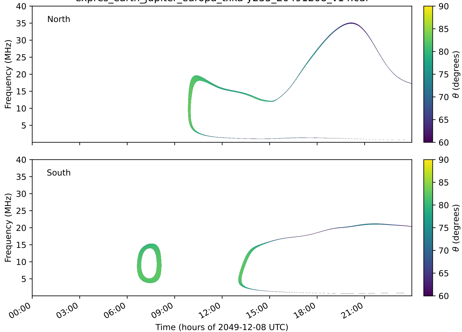
expres_earth_jupiter_europa_txka-y235_20491208_v14.cdf
