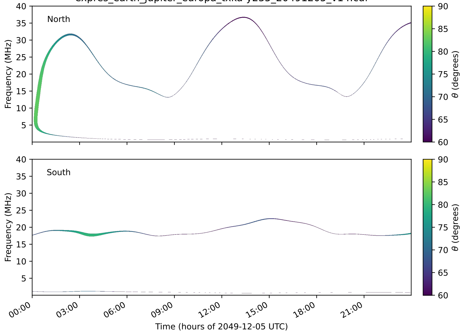
expres_earth_jupiter_europa_txka-y235_20491205_v14.cdf
