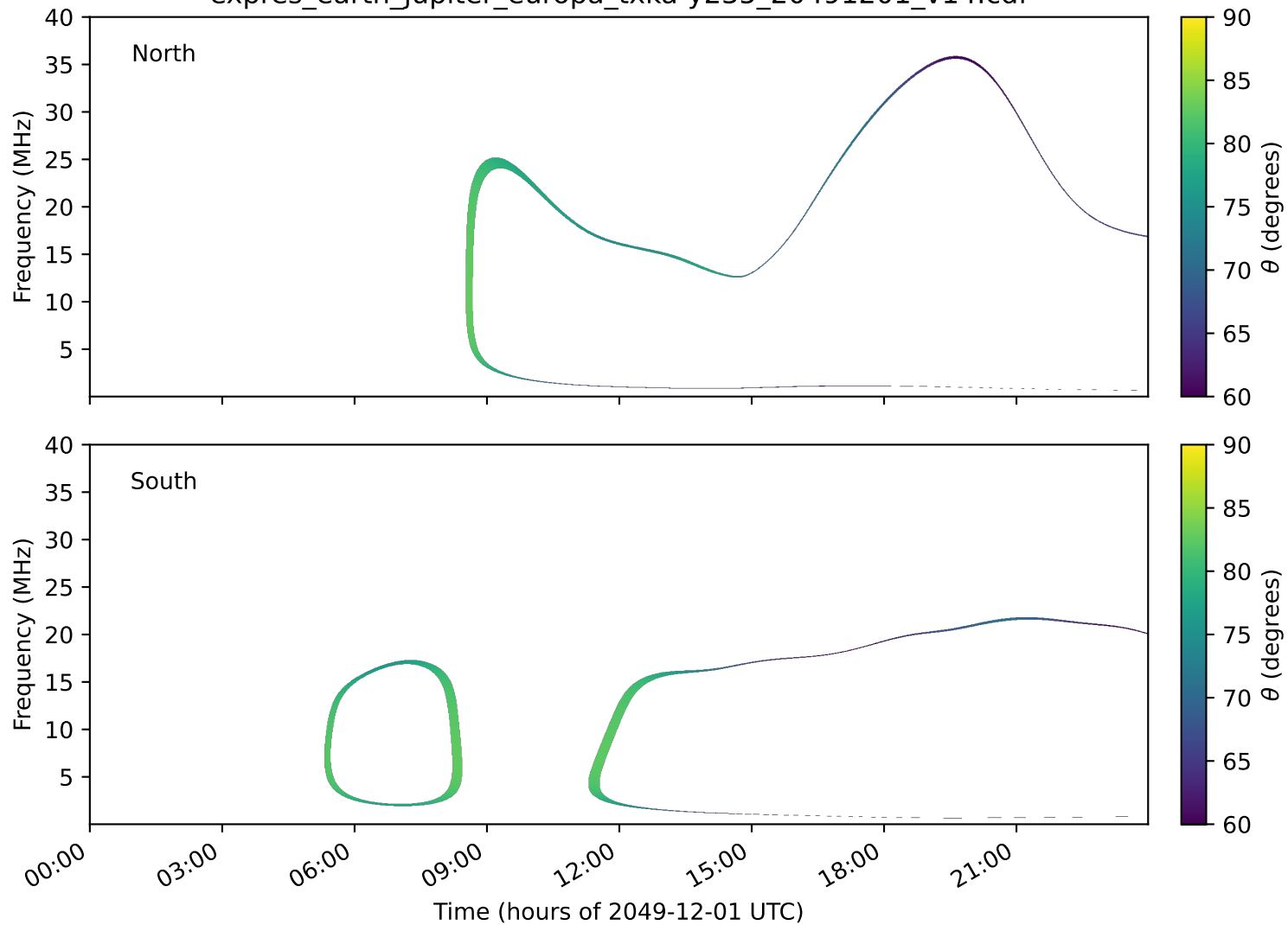
expres_earth_jupiter_europa_txka-y235_20491201_v14.cdf
