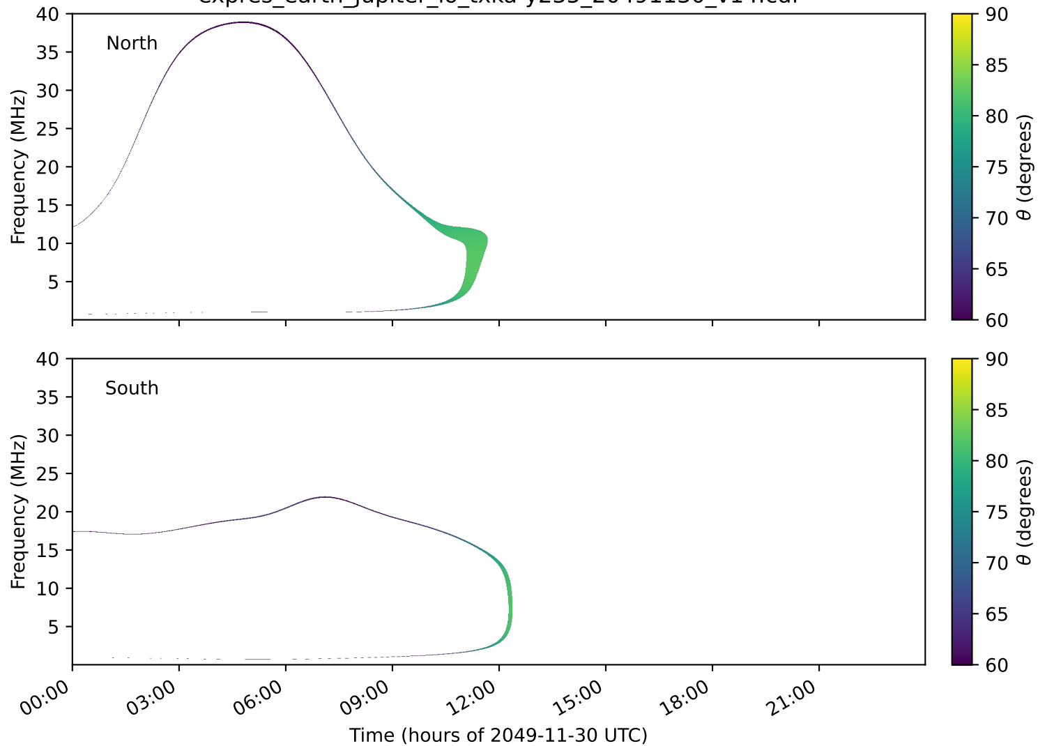
expres_earth_jupiter_io_txka-y235_20491130_v14.cdf
