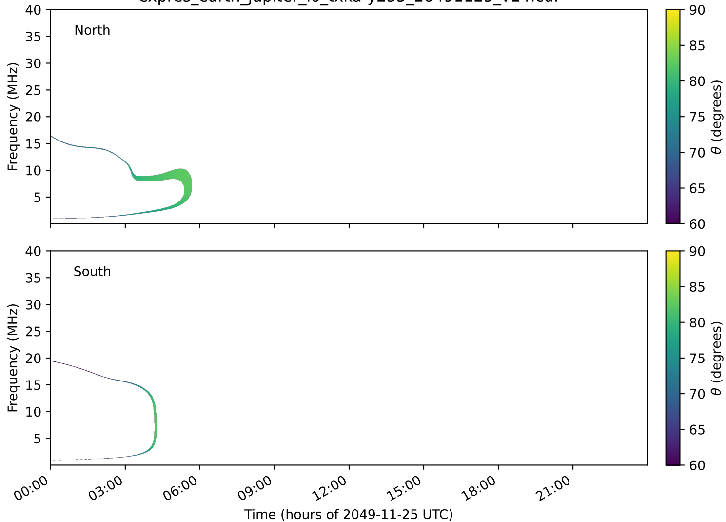
expres_earth_jupiter_io_txka-y235_20491125_v14.cdf
