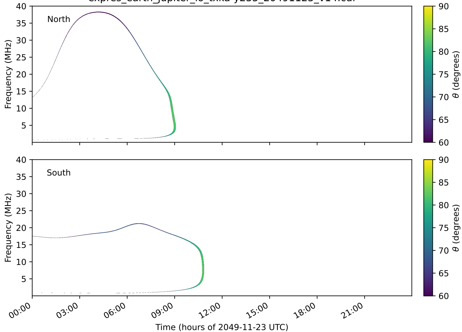
expres_earth_jupiter_io_txka-y235_20491123_v14.cdf
