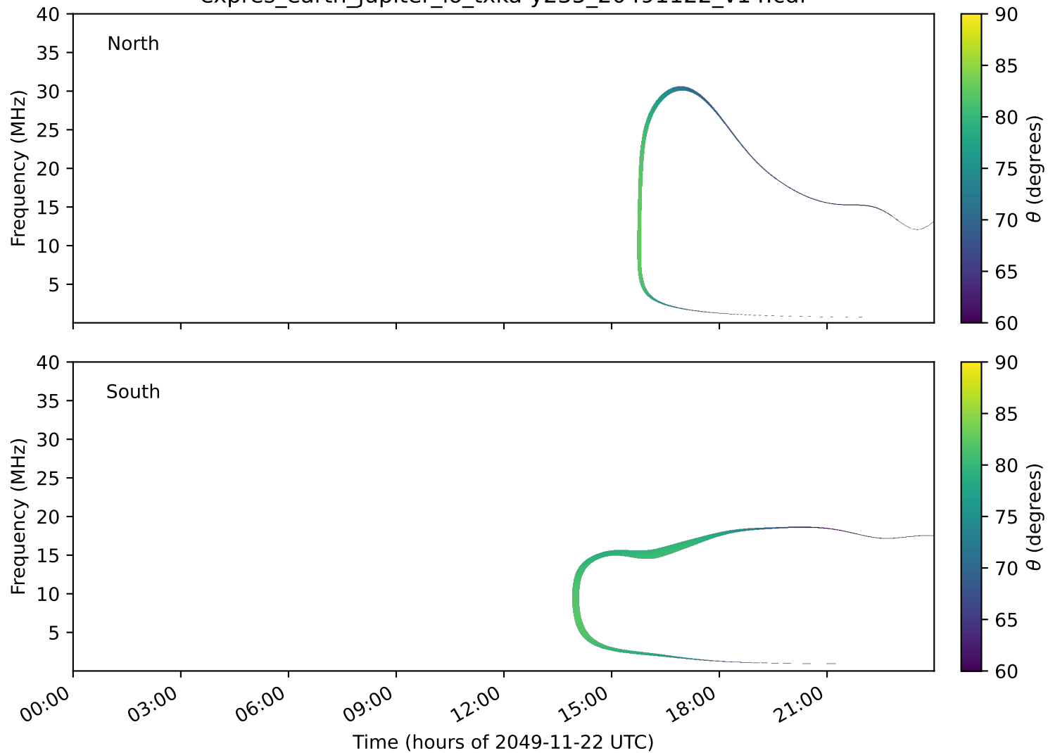
expres_earth_jupiter_io_txka-y235_20491122_v14.cdf
