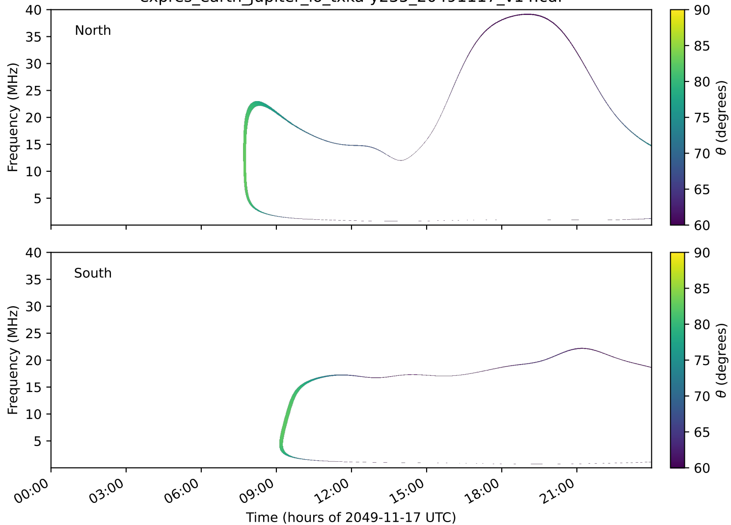
expres_earth_jupiter_io_txka-y235_20491117_v14.cdf
