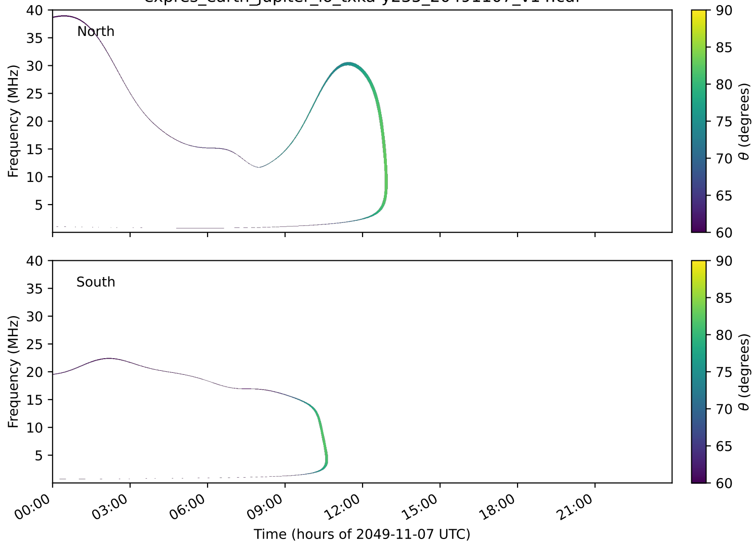
expres_earth_jupiter_io_txka-y235_20491107_v14.cdf
