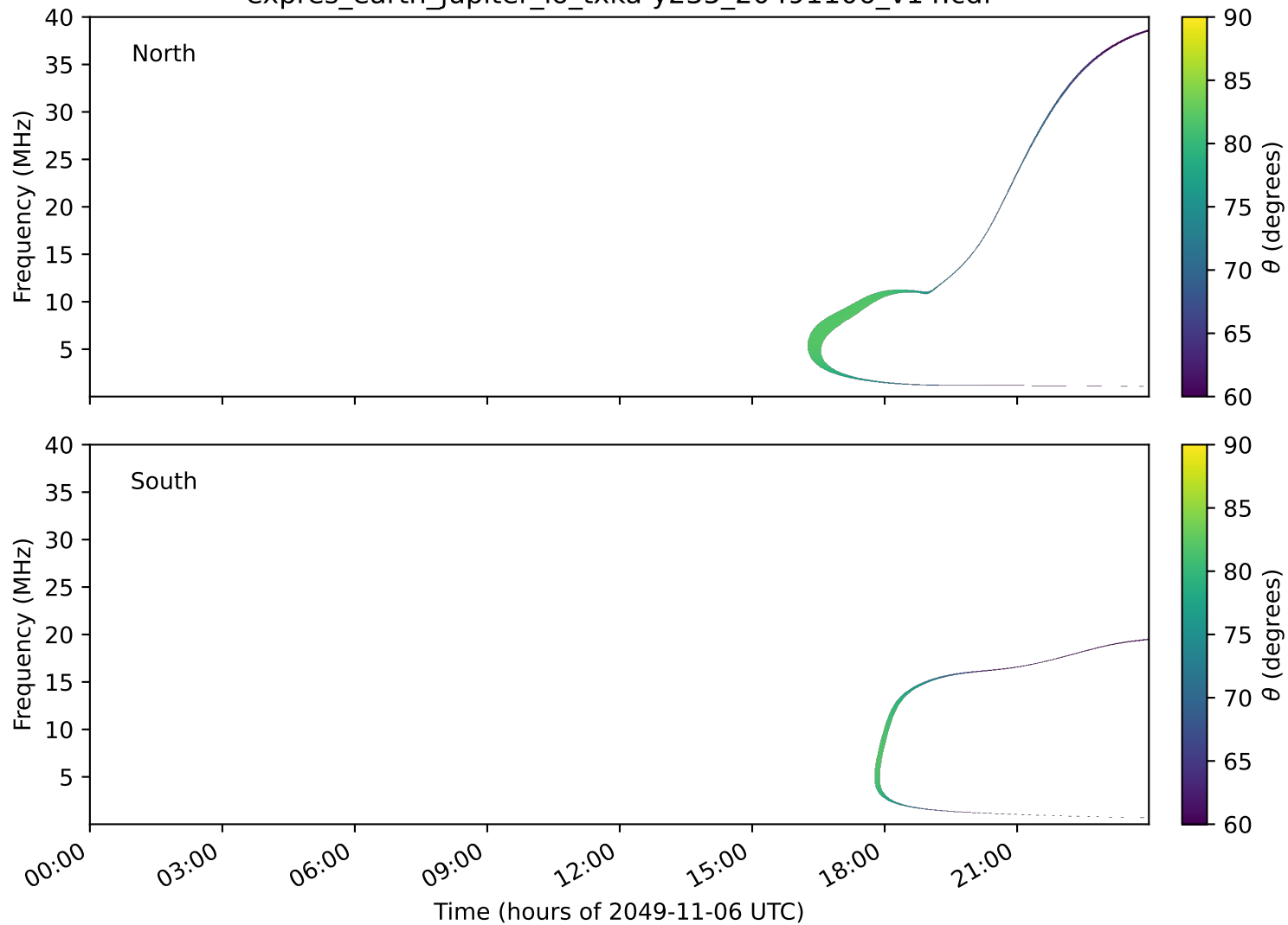
expres_earth_jupiter_io_txka-y235_20491106_v14.cdf
