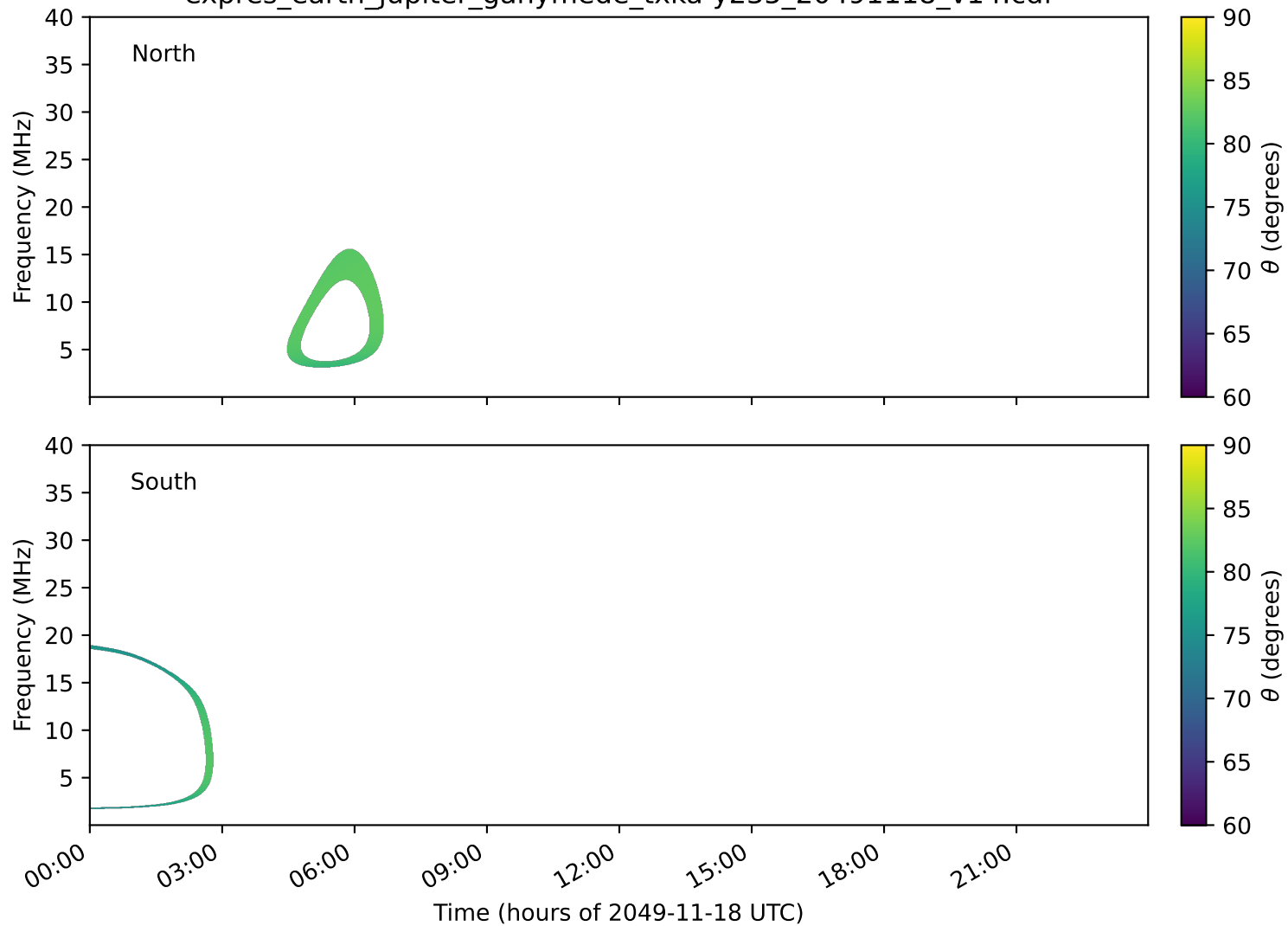
expres_earth_jupiter_ganymede_txka-y235_20491118_v14.cdf
