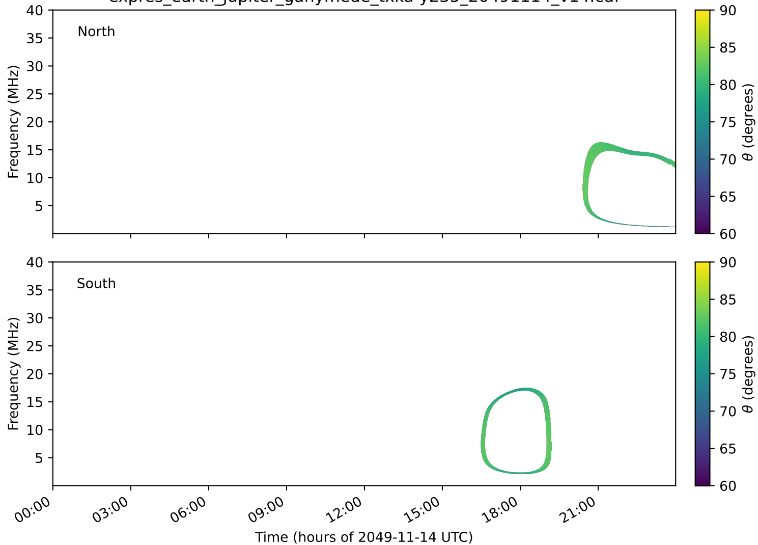
expres_earth_jupiter_ganymede_txka-y235_20491114_v14.cdf
