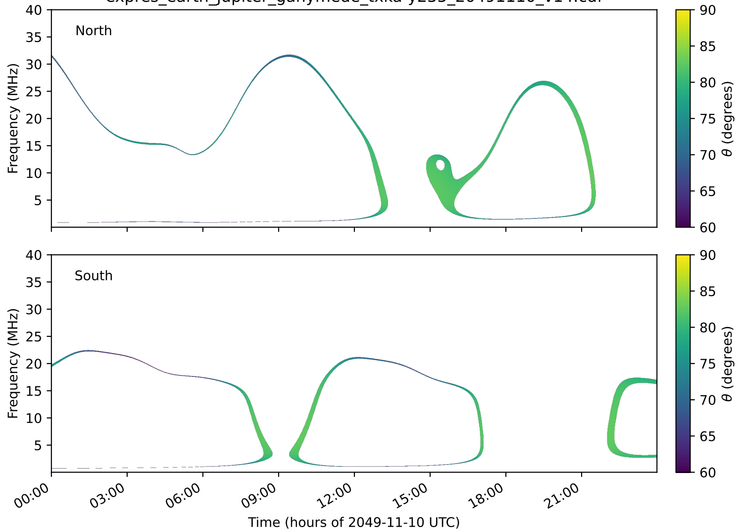
expres_earth_jupiter_ganymede_txka-y235_20491110_v14.cdf
