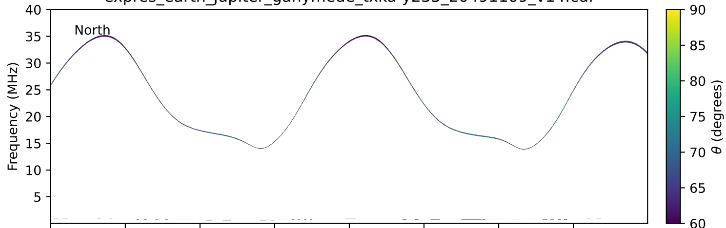
expres_earth_jupiter_ganymede_txka-y235_20491109_v14.cdf
