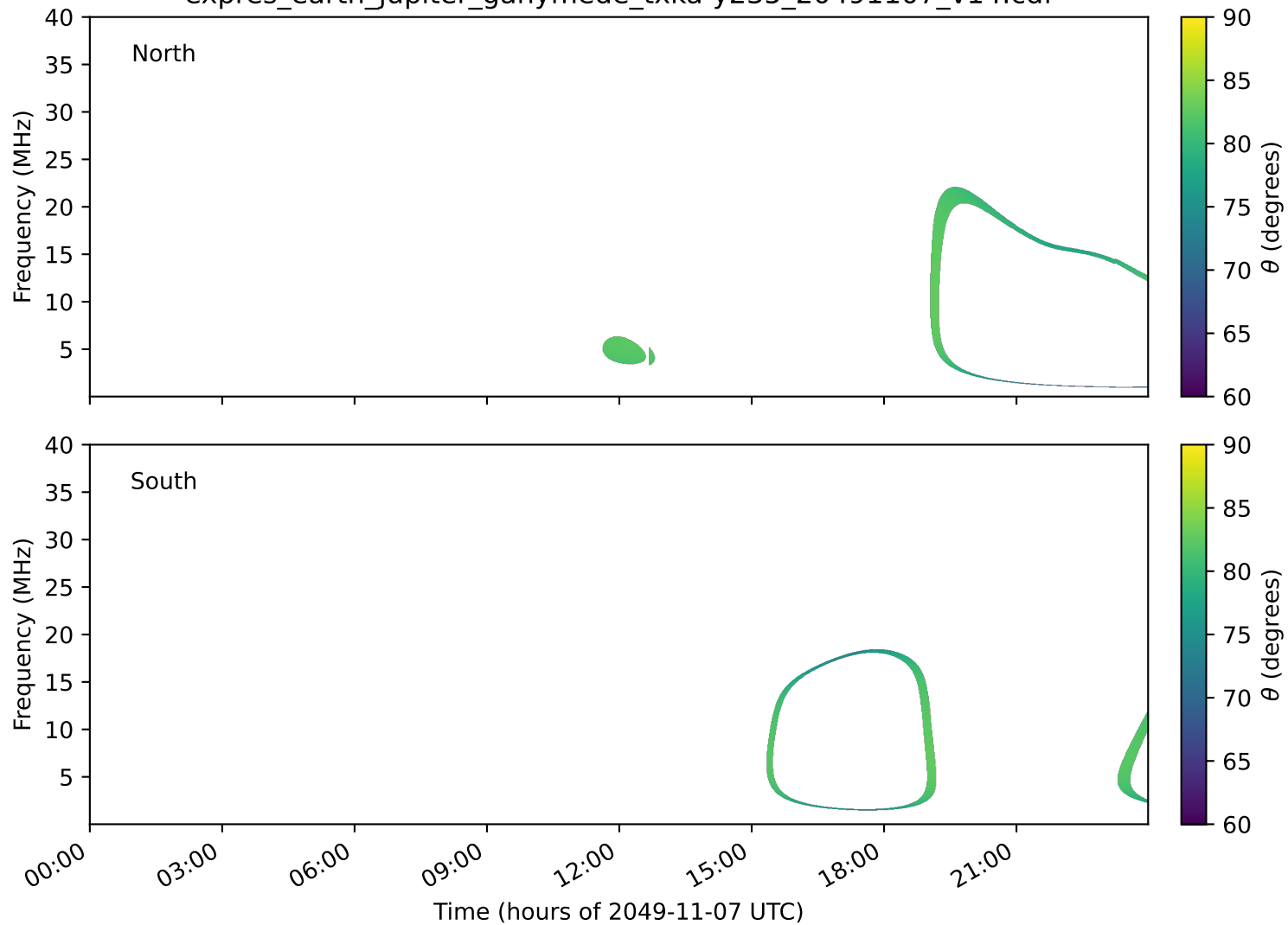
expres_earth_jupiter_ganymede_txka-y235_20491107_v14.cdf
