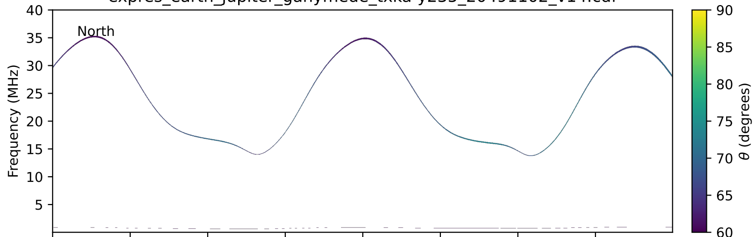
expres_earth_jupiter_ganymede_txka-y235_20491102_v14.cdf
