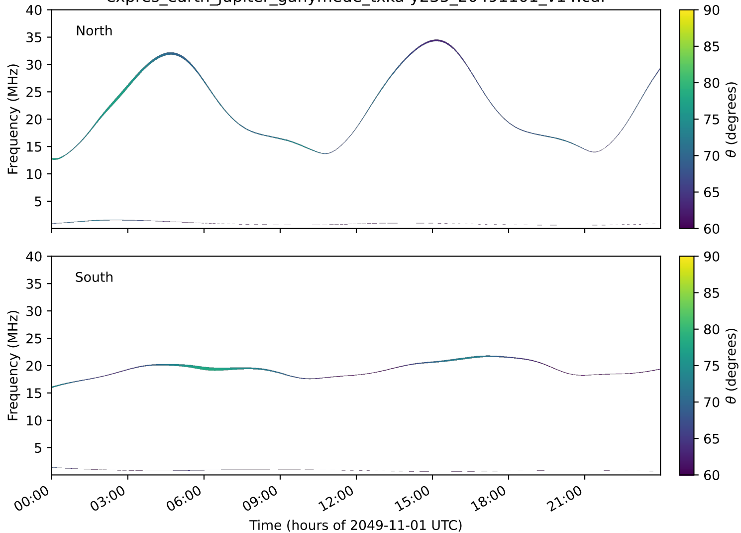
expres_earth_jupiter_ganymede_txka-y235_20491101_v14.cdf
