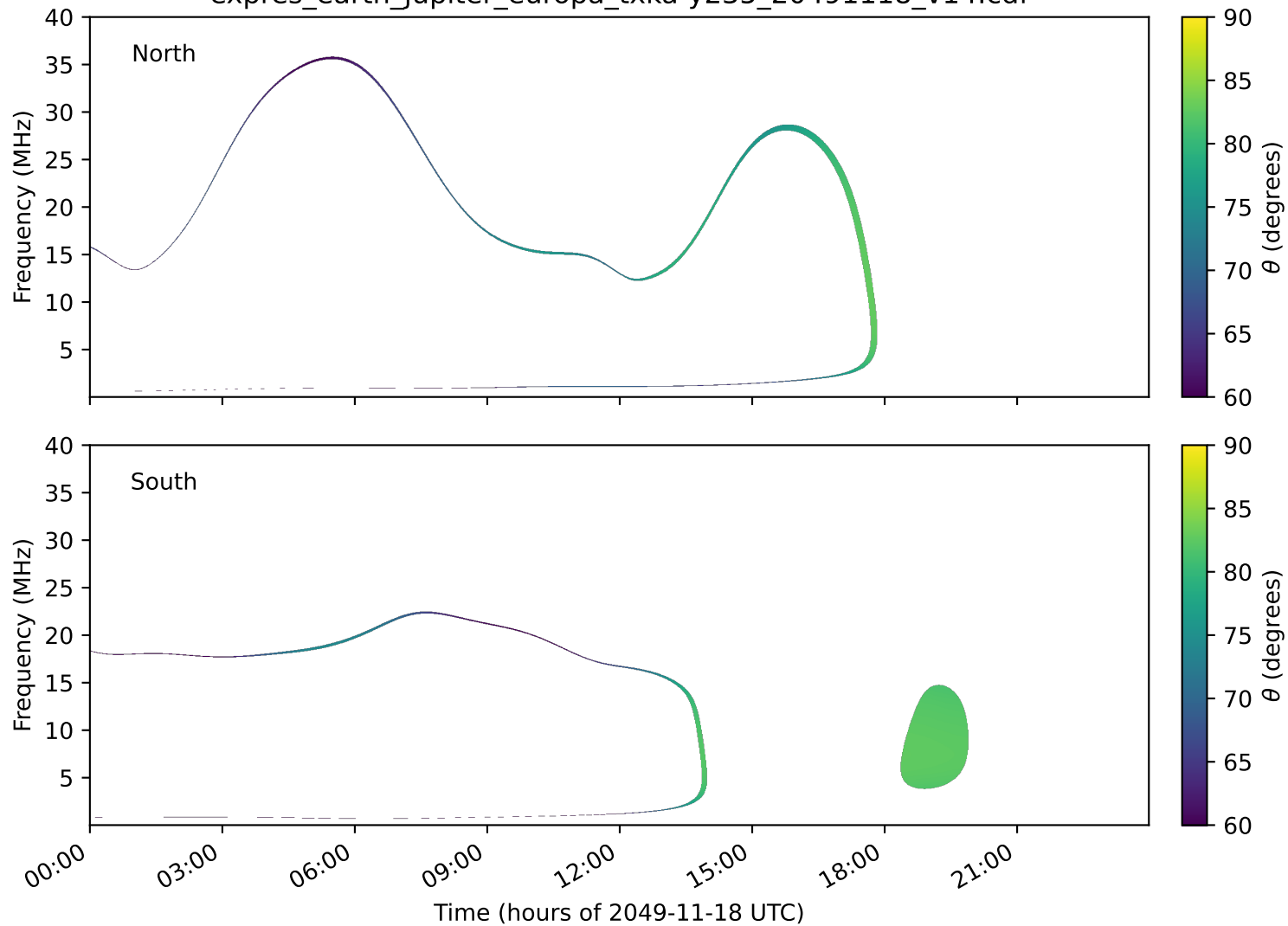
expres_earth_jupiter_europa_txka-y235_20491118_v14.cdf
