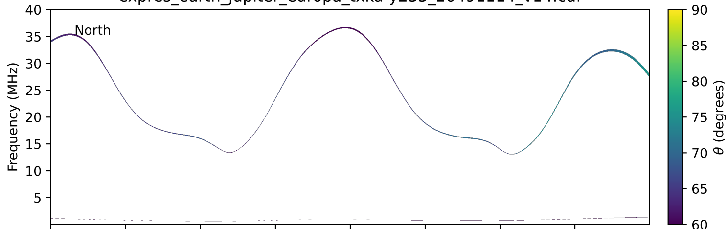
expres_earth_jupiter_europa_txka-y235_20491114_v14.cdf
