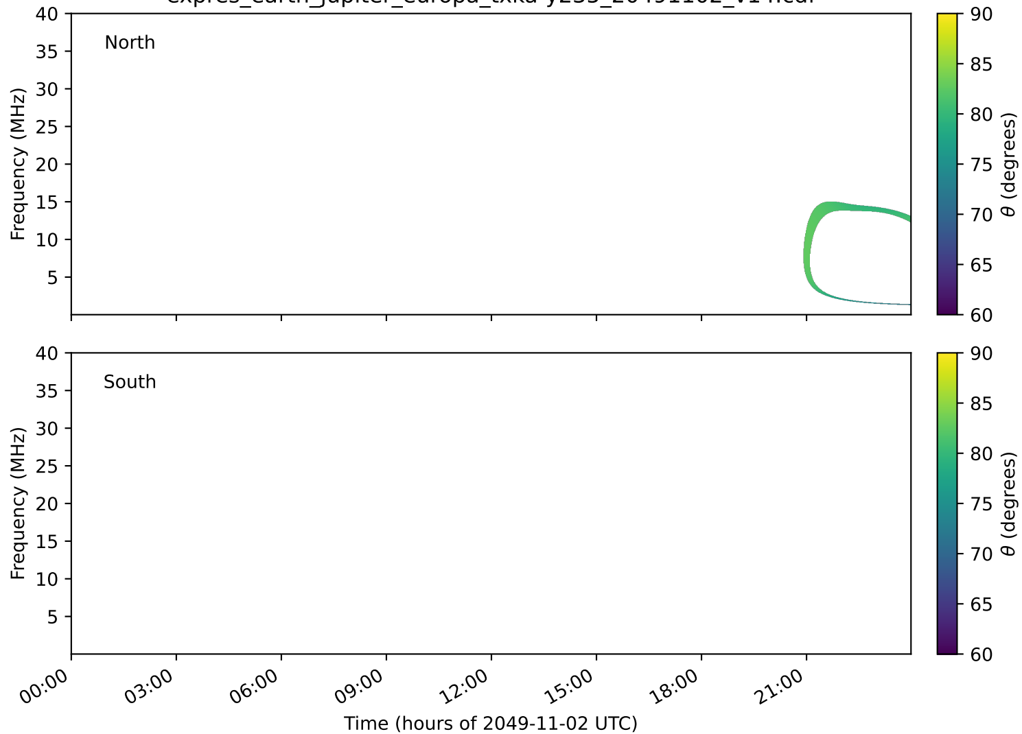
expres_earth_jupiter_europa_txka-y235_20491102_v14.cdf
