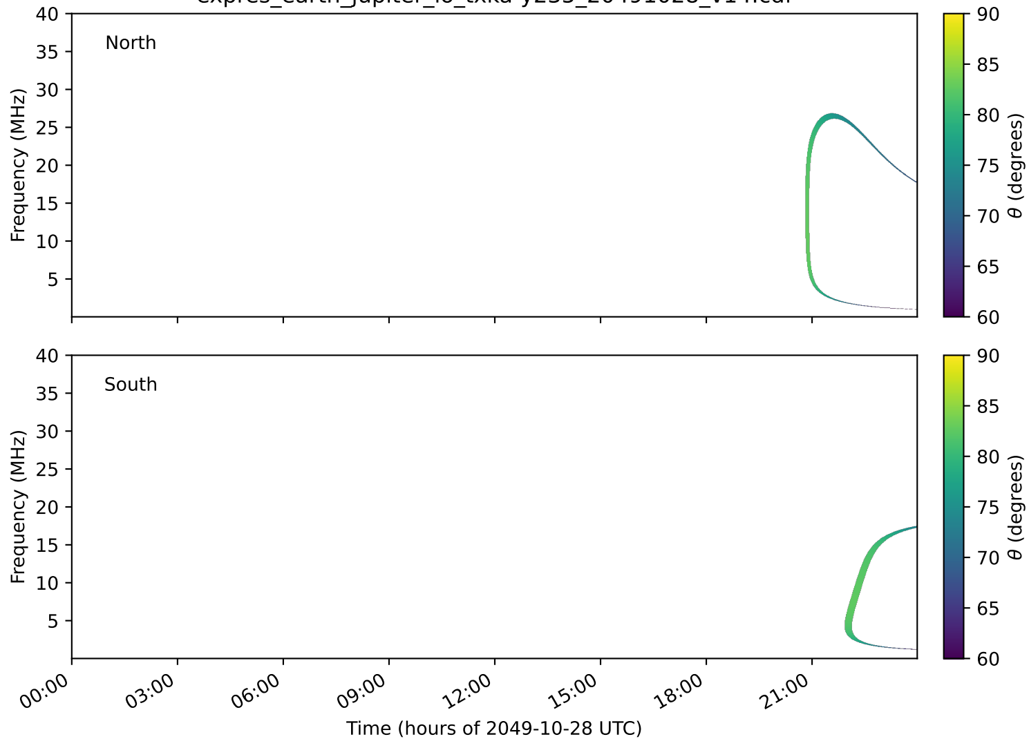
expres_earth_jupiter_io_txka-y235_20491028_v14.cdf
