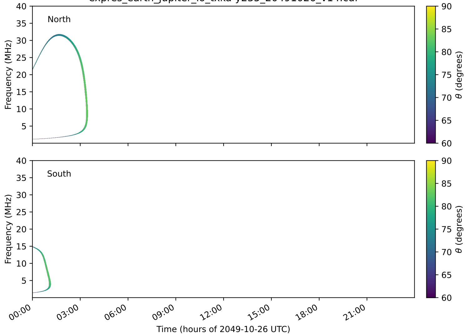
expres_earth_jupiter_io_txka-y235_20491026_v14.cdf
