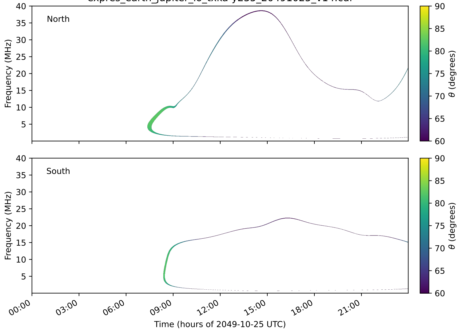
expres_earth_jupiter_io_txka-y235_20491025_v14.cdf
