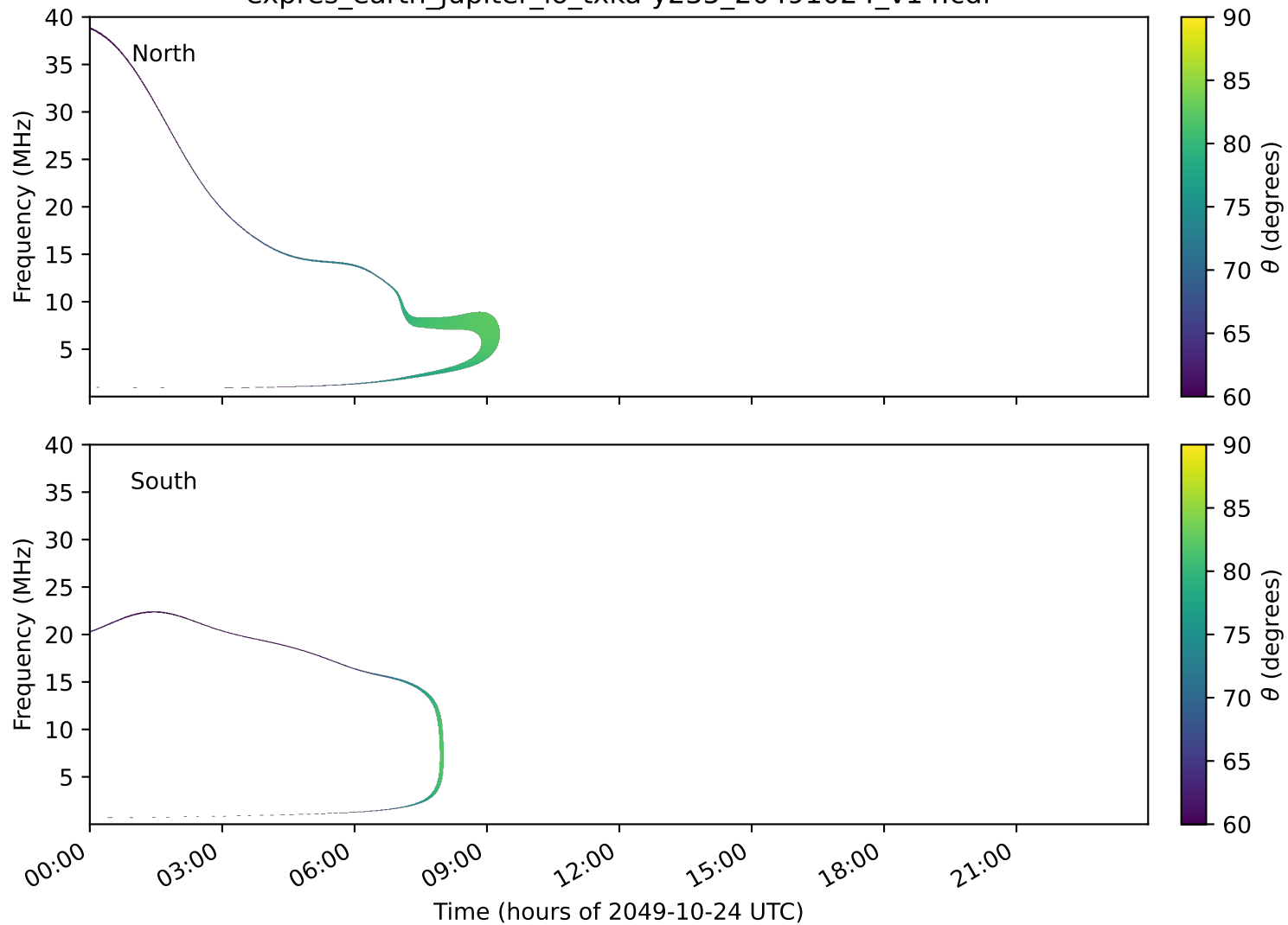
expres_earth_jupiter_io_txka-y235_20491024_v14.cdf
