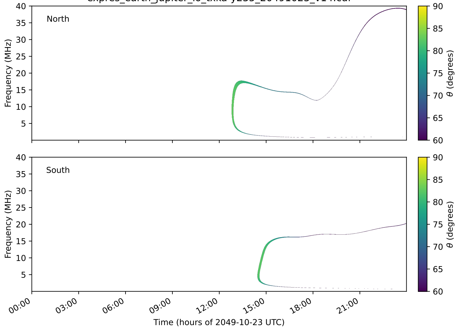
expres_earth_jupiter_io_txka-y235_20491023_v14.cdf
