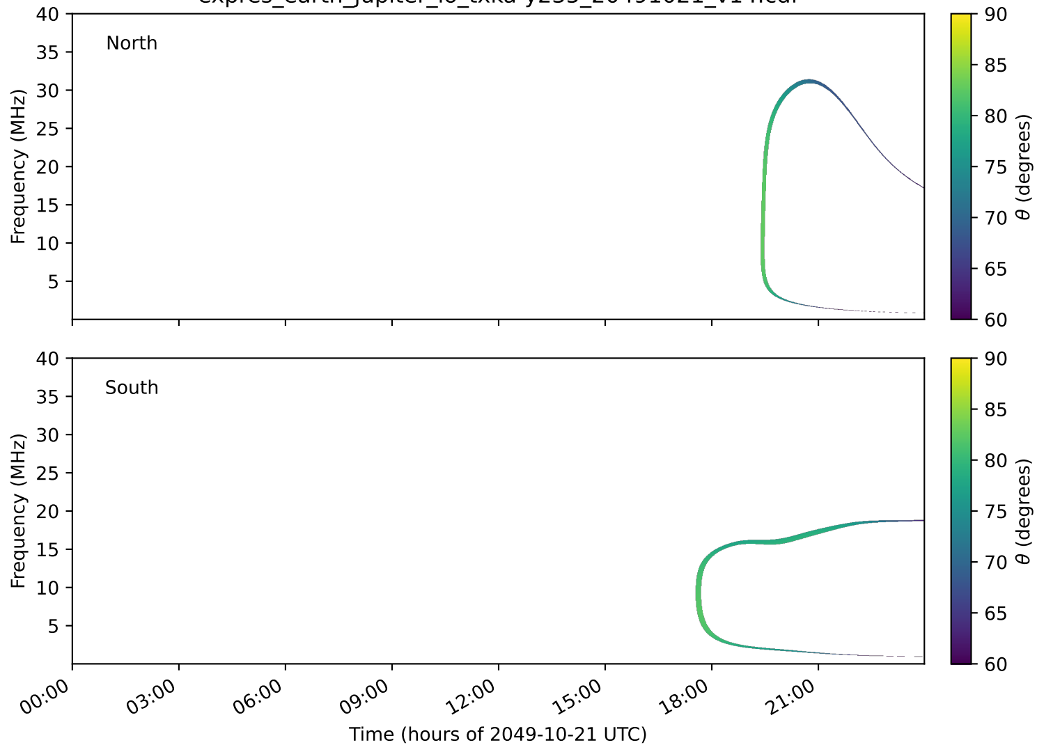
expres_earth_jupiter_io_txka-y235_20491021_v14.cdf
