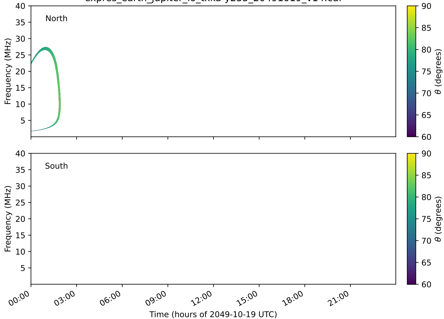
expres_earth_jupiter_io_txka-y235_20491019_v14.cdf
