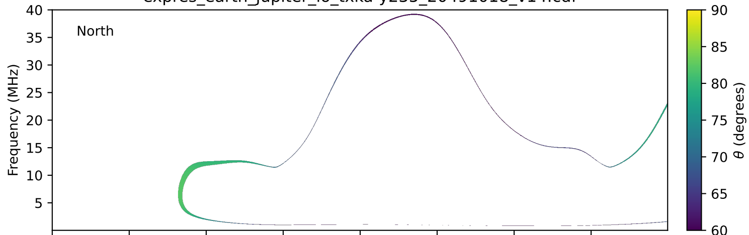
expres_earth_jupiter_io_txka-y235_20491018_v14.cdf
