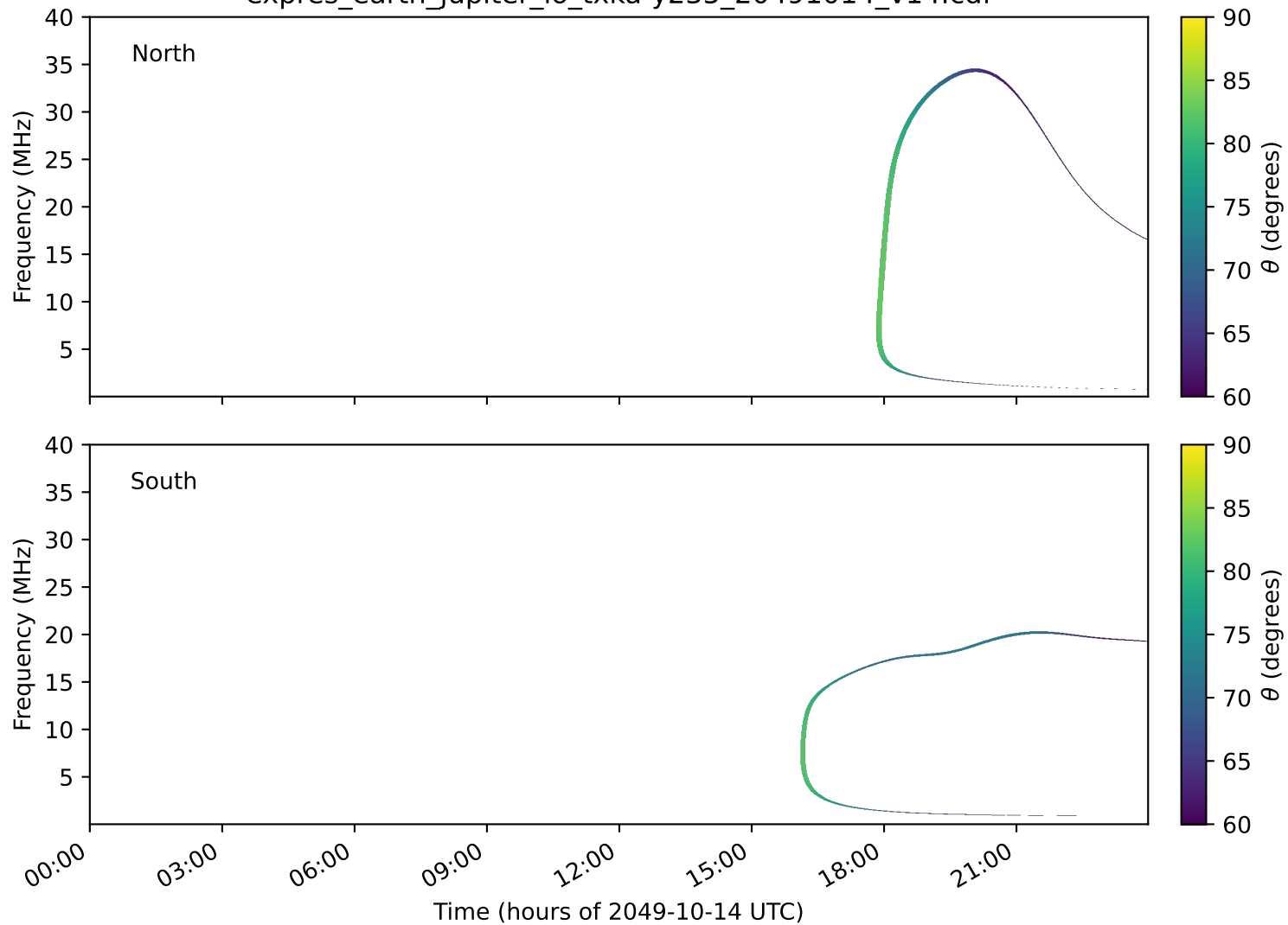
expres_earth_jupiter_io_txka-y235_20491014_v14.cdf
