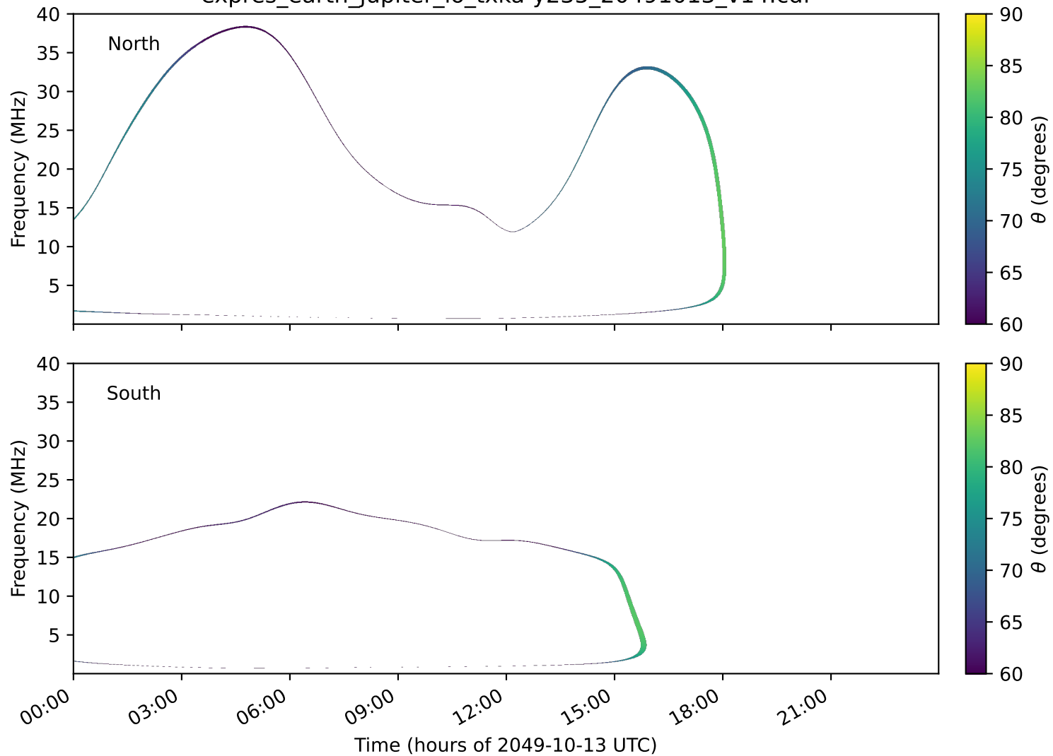
expres_earth_jupiter_io_txka-y235_20491013_v14.cdf
